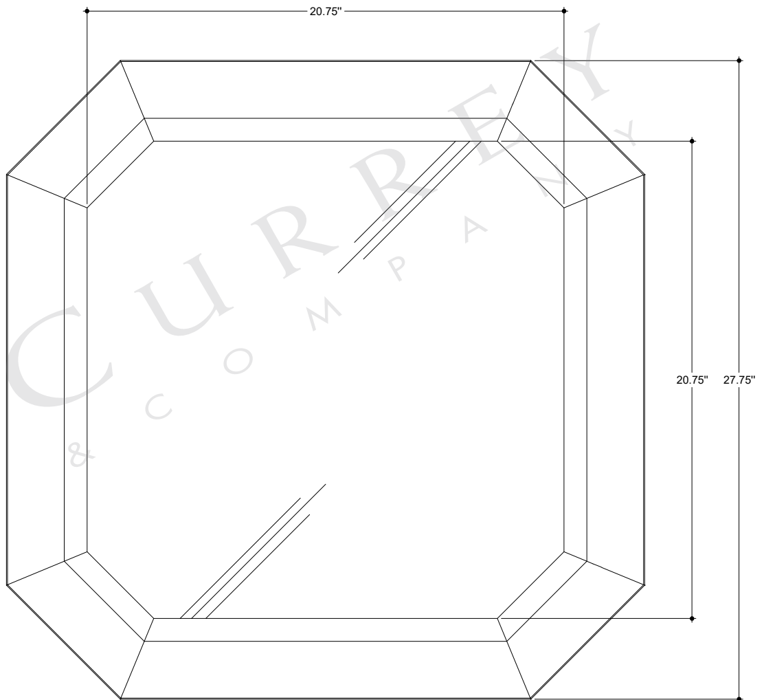
FRONT VIEW
